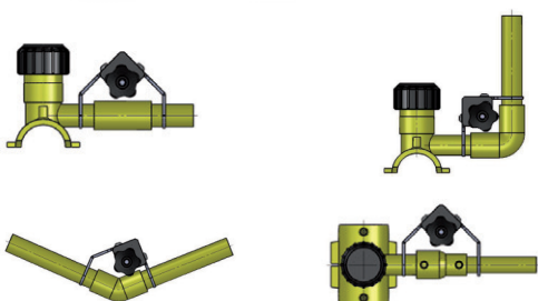
EFrac Clamp Set for 63mm Diameter
